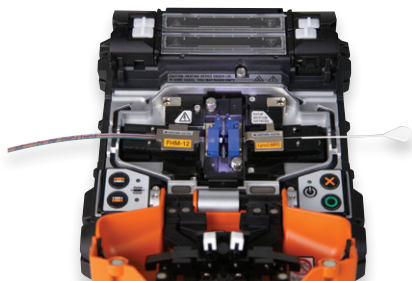
Shown with Optional Lynx2-MPO CustomFit® Splice-On Connector
