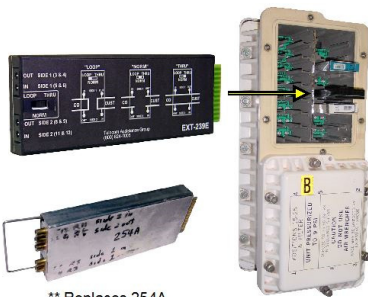
Test Boards & Extenders Test Kits & T1 Test Cords
